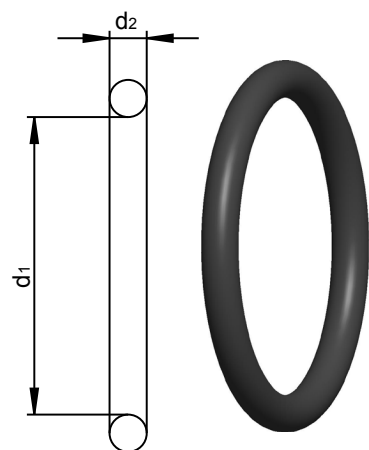
Fig.1, O-ring
