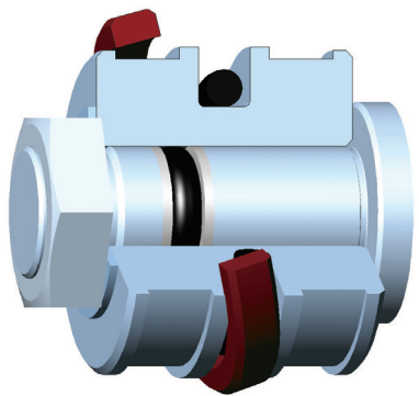
Fig. 2, Installation of XHPU seals is made with simple or no tools
