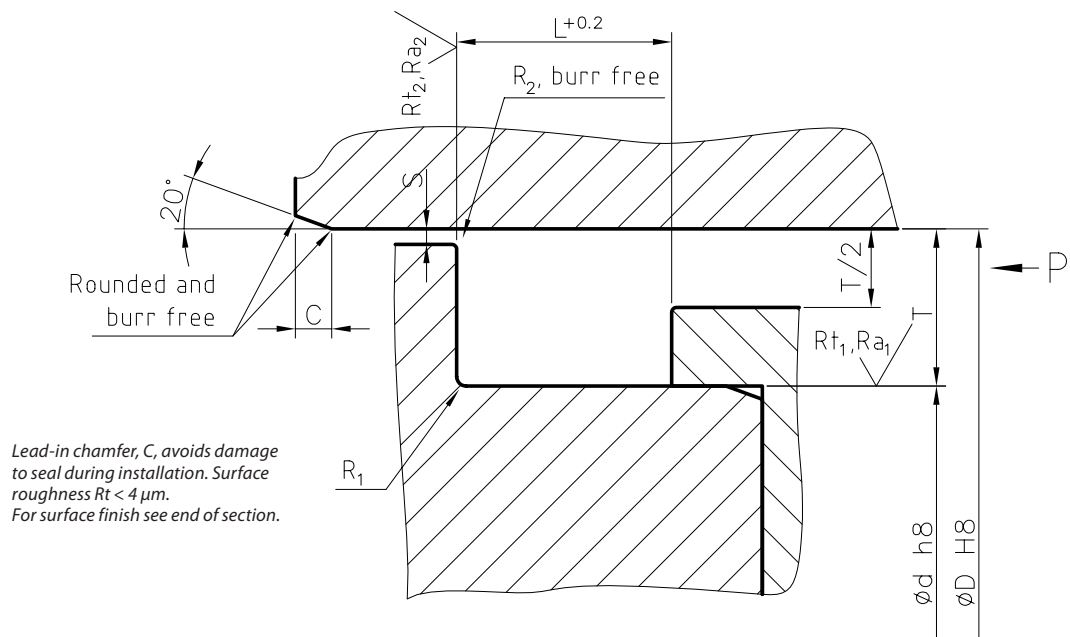
Fig. 13, Housing for piston seals K03-S, K19-F.
