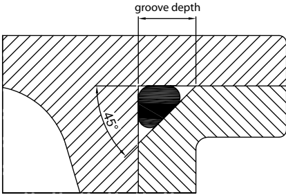
Fig. 18, Triangular groove
