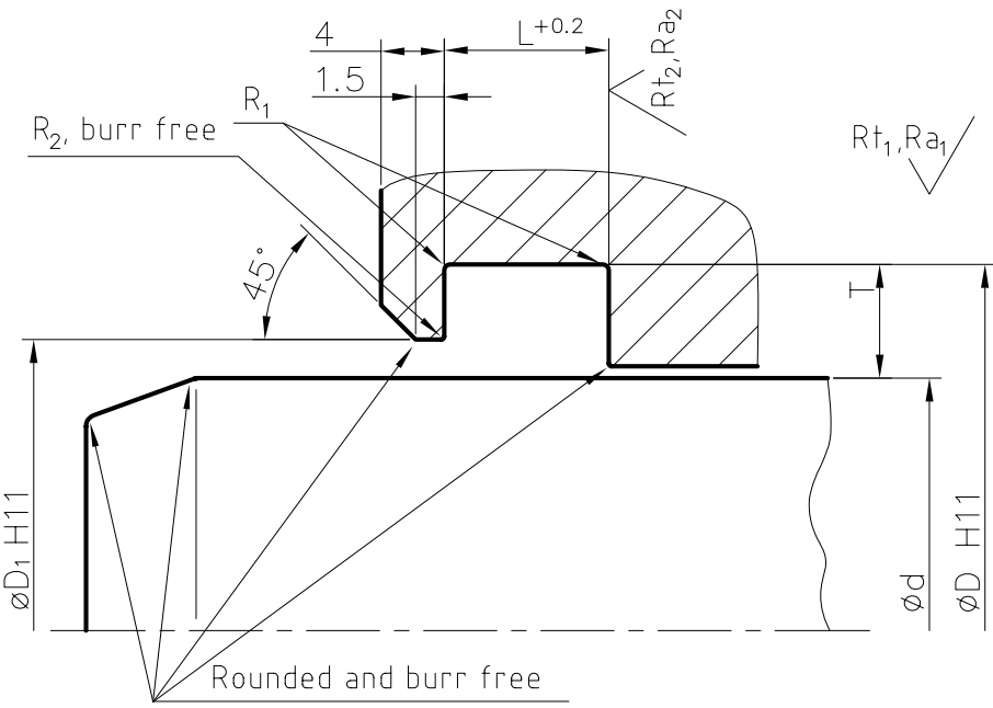
Fig. 4, Housing for wiper A26, A27.
