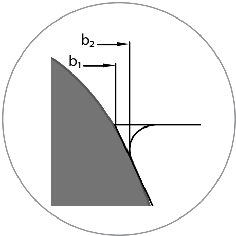
Fig. 17, Detail of trapezoidal groove
