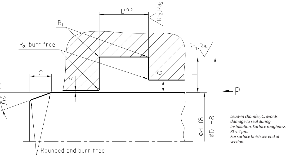
Fig. 7, Housing for rod seals S01, S02, S03, S04, S05, S17, S18, S24
