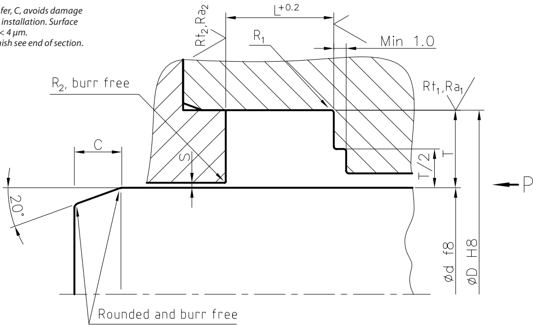
Fig. 8, Housing for rod seals S03-S, S19-S
