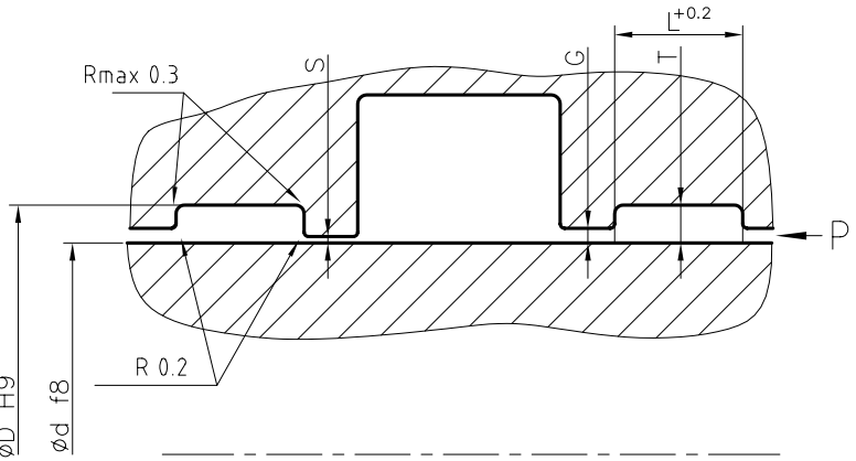
Fig. 18, Housing for guide ring F01 (rod).
