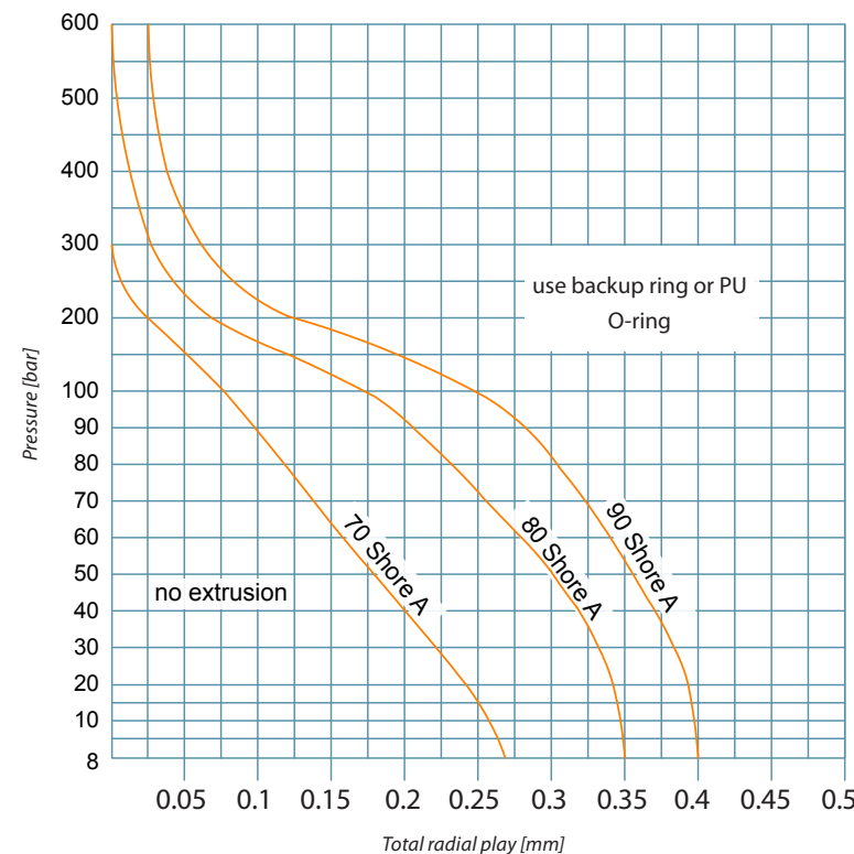
Fig. 2, Pressure resistance
