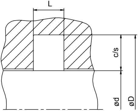
Fig 6, Housing for rotary seal
