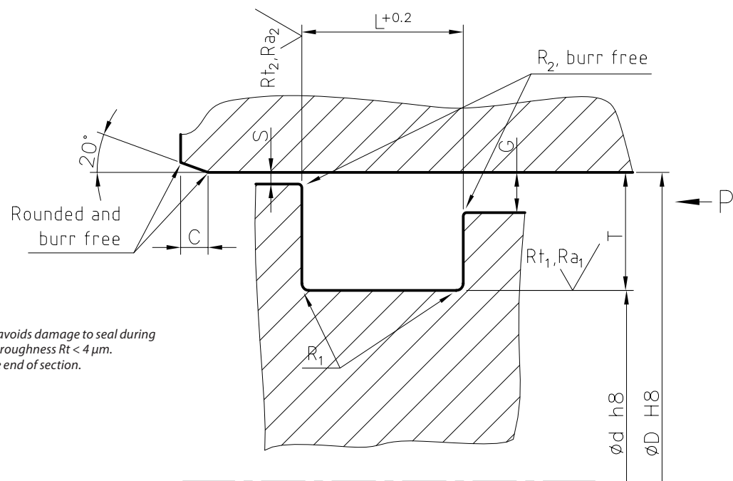
Fig. 10, Housing for piston seals K01
