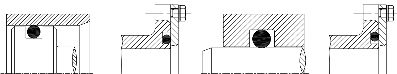
Fig. 7, Internal groove
