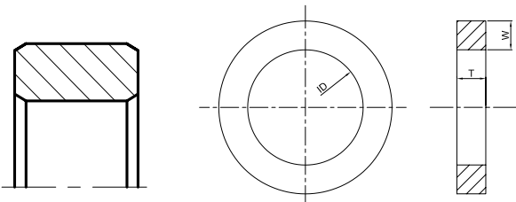
Fig. 24, Profile R14 with chamfer.
