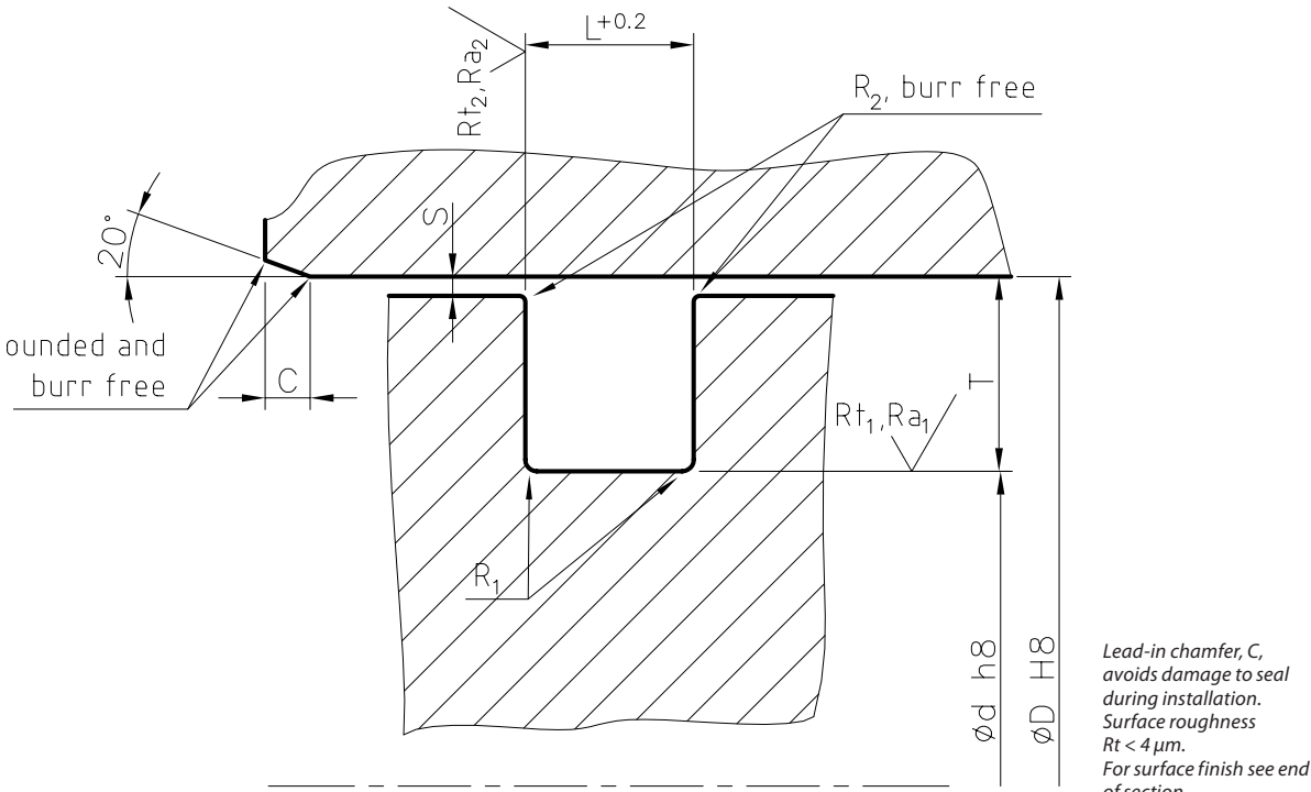
Fig. 11, Housing for piston seals K08.
