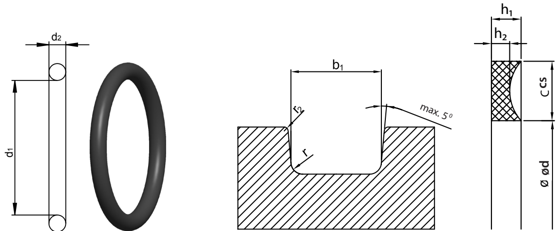
Fig. 12, O-ring
