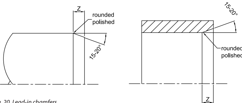
Fig. 20, Lead-in chamfers
