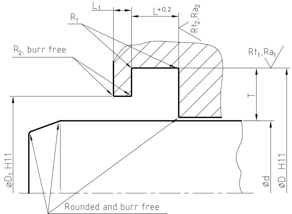
Fig. 3, Housing for wiper A12.
