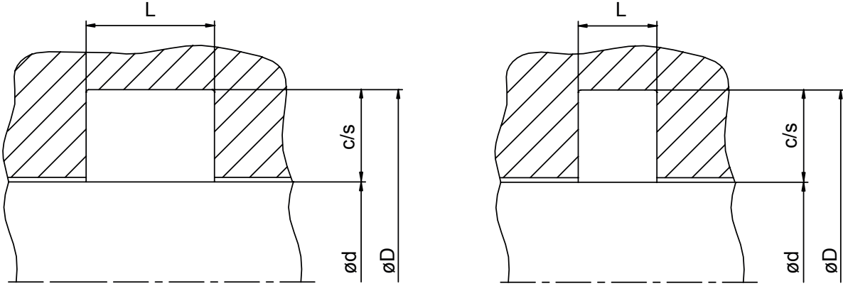
Fig. 2, Housings for rod seals
