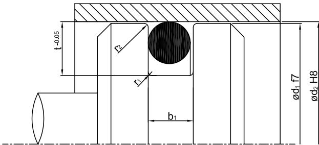
Fig. 19, Pneumatic floating fit
