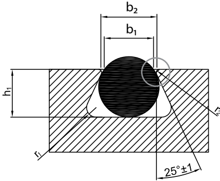
Fig. 16, Trapezoidal groove
