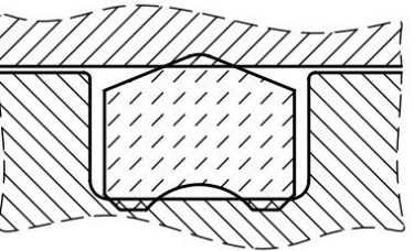
Fig 23, Similar groove with K35-P
