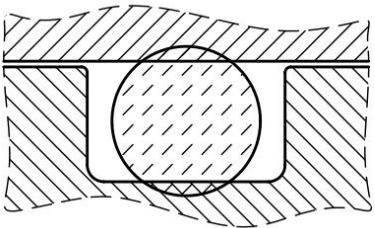
Fig 22, O-ring groove with O-ring
